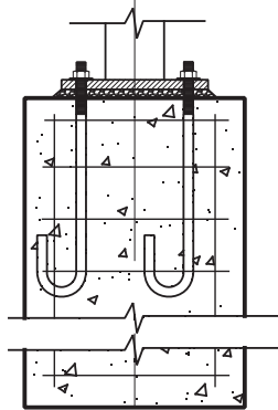
USING J-BOLTS
